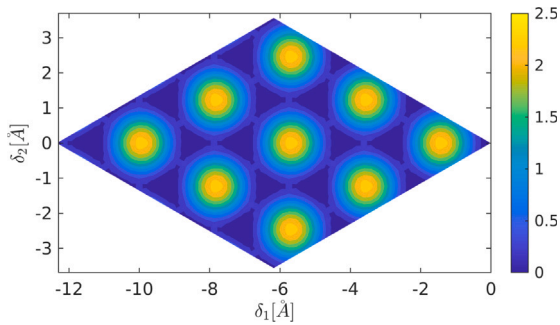
Fig. 2. GSFE of AB stacking in \text{meV \AA}^{-2} . The minima and maxima correspond to the AB and AA stackings, respectively. Parametrizations KC-1 and KC-2 yield nearly identical GSFEs.
