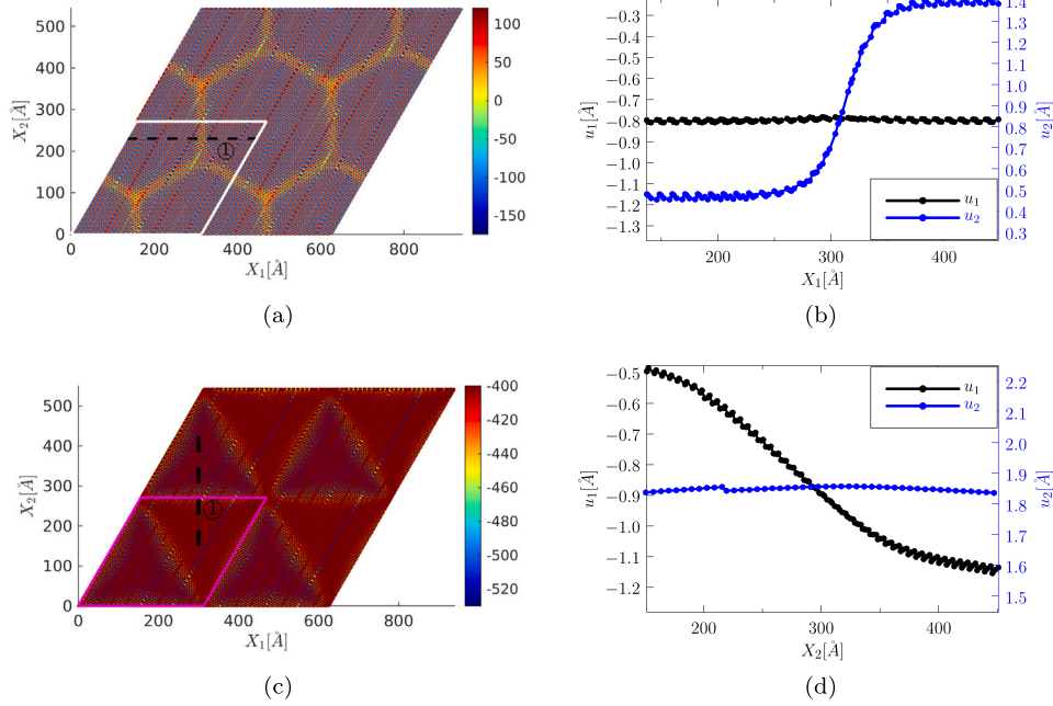
Fig. 4. Atomic reconstruction in a large-twist ( 21.786789^\circ + 0.170076^\circ ) BG using the KC-1 (top row) and the KC-2 (bottom row) models. (a), (c) Plots of atomic energy density [ \text{meV \AA}^{-2} ] show a honeycomb and a triangular network of interface dislocations. (b), (d) Line plots of the displacement components u_1 and u_2 , measured along the dashed lines in (a) and (c). The displacements are measured relative to the untwisted \Sigma 7 configuration.
