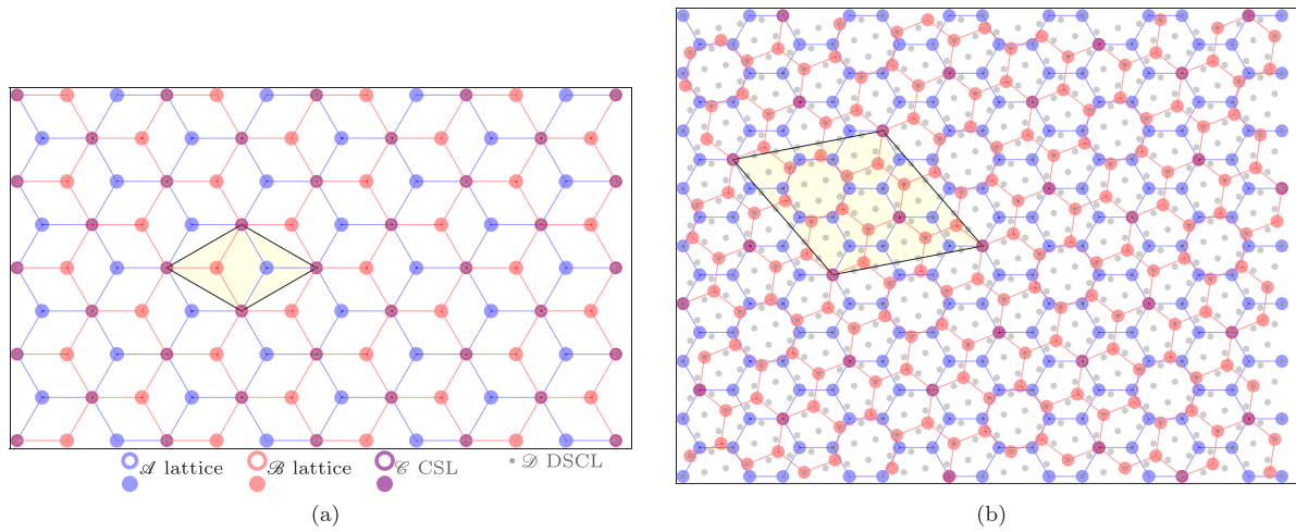
Fig. 7. (a) AB-stacked ( 0^\circ twist) bilayer graphene forming a \Sigma = 1 moiré. (b) 21.786789^\circ twisted BG resulting in a \Sigma = 7 moiré. Open circles represent the second basis atom of graphene. The two graphene lattices, \mathcal{A} and \mathcal{B} , are shown in blue and red, while the moiré superlattice ( \mathcal{C} ) and the DSCL ( \mathcal{D} ) are shown in purple and gray, respectively. The highlighted region represents a unit cell of \mathcal{C} . The ratio of the unit cell size of the moiré superlattice to that of the graphene lattice and the corresponding ratio between the graphene lattice and \mathcal{D} are equal to \Sigma . (For interpretation of the references to color in this figure legend, the reader is referred to the web version of this article.)
