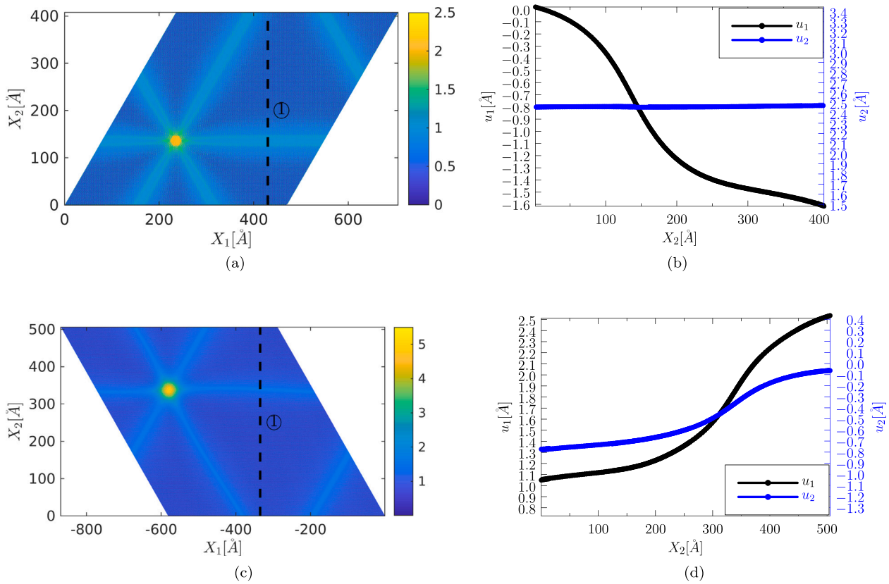
Fig. 1. Atomic reconstruction in a BG under a small twist (top row) and a small heterostrain (bottom row). (a), (c) Plots of atomic energy density [ \text{meV \AA}^{-2} ] show a triangular network of interface dislocations. The dislocation lines separate triangular domains of low-energy AB-stacking. (b), (d) Line plots of the displacement components u_1 and u_2 , measured along the dashed lines in (a) and (c). The displacements are measured relative to the untwisted AB-stacked configuration.
