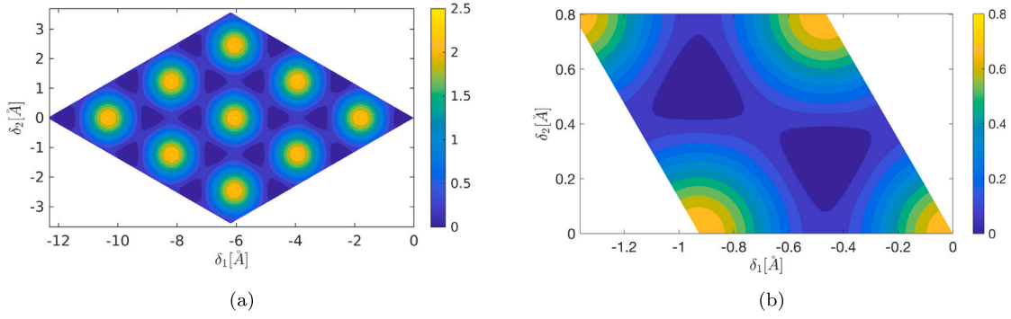
Fig. 12. Plots of e_{\text{vdW}} for (a) AB-stacked \Sigma 1 and (b) \Sigma 7 configurations, computed using (15) and plotted such that the minimum is zero.
