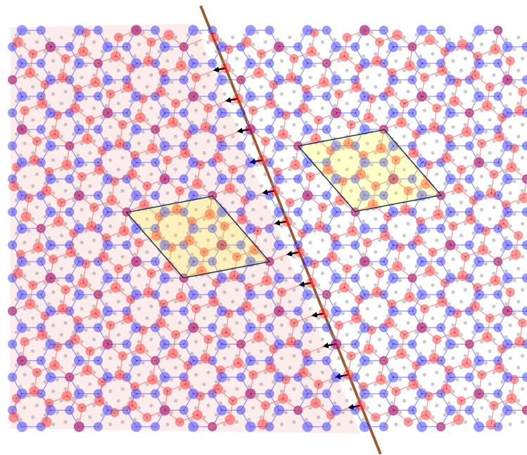
Fig. 8. Translational invariance of a 21.786789^\circ twisted BG. Translating the shaded region of the red lattice by a DSCL vector leaves the interface structure invariant and results in a shift in the CSL. (For interpretation of the references to color in this figure legend, the reader is referred to the web version of this article.)
