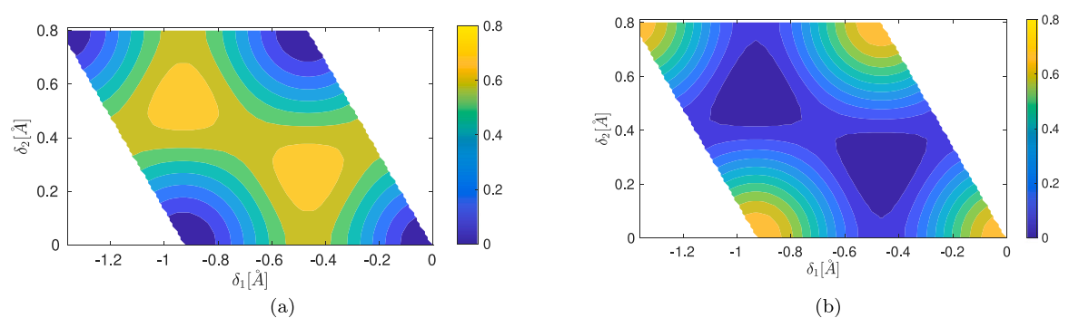
Fig. 9. GSFE [ \text{meV } \text{\AA}^{-2} ] plots of \Sigma 7 21.786789^\circ twisted BG, computed in LAMMPS using (a) the KC-1 parametrization at 26% out-of-plane compression, and (b) the KC-2 parametrization at 39% out-of-plane compression.
