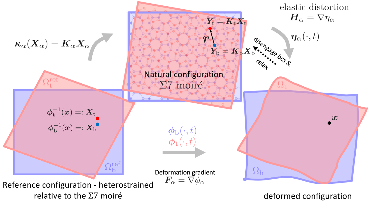
Fig. 11. A schematic of the reference (left), natural (middle), and deformed (right) configurations of the GFK model.
