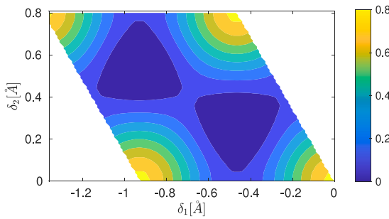
Fig. 10. Density functional theory-generated GSFE [ \text{meV } \text{Å}^{-2} ] of a \Sigma 7 21.786789° twisted BG at 26% out-of-plane compression.
