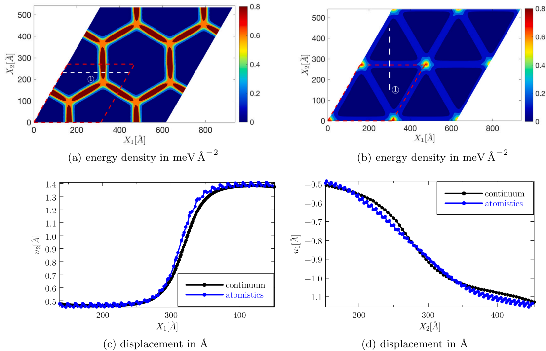
Fig. 15. Structural relaxation in a 21.95686492519 Å large-twist BG using the KC-1 and KC-2 parametrizations. The energy density plots in (a) and (b) highlight the honeycomb and the triangular network of interface dislocations, corresponding to KC-1 and KC-2 models, respectively. (c) and (d) compare the displacement across the dashed lines predicted by the atomistic and the GFK models.
