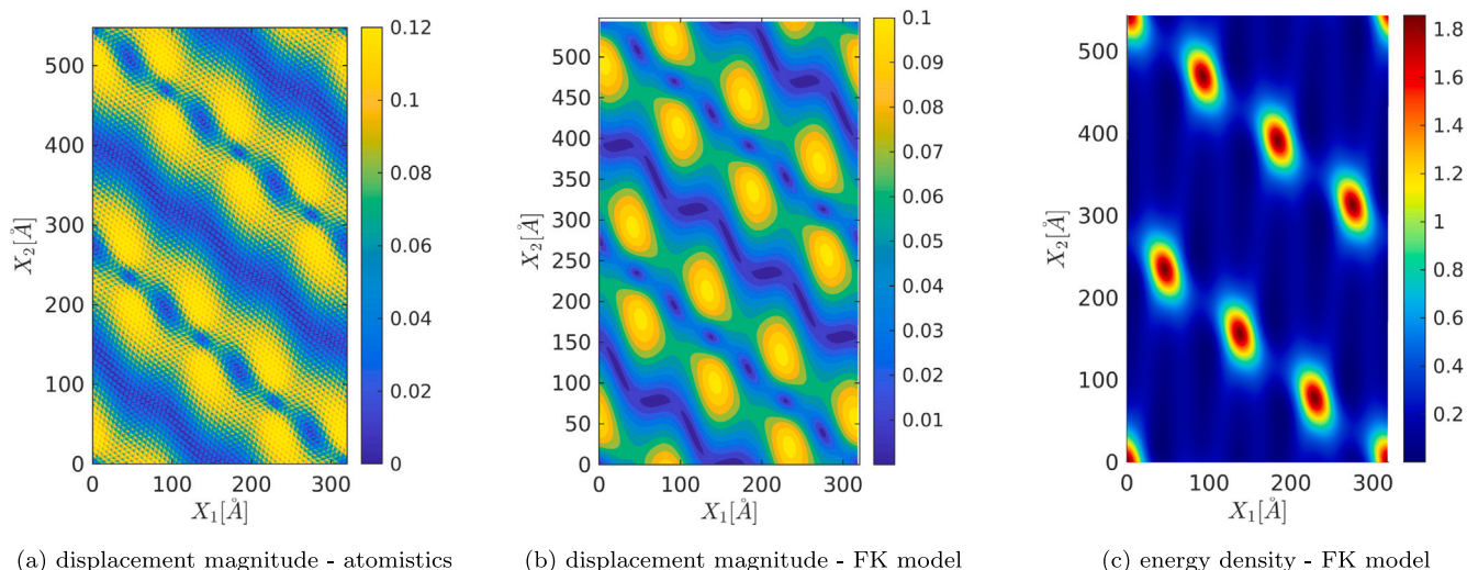
Fig. 16. Simulation results of a heterostrained 21.786789^\circ large-twist BG. The units of displacement and energy density are \text{\AA} and \text{meV}\text{\AA}^{-2} , respectively.
