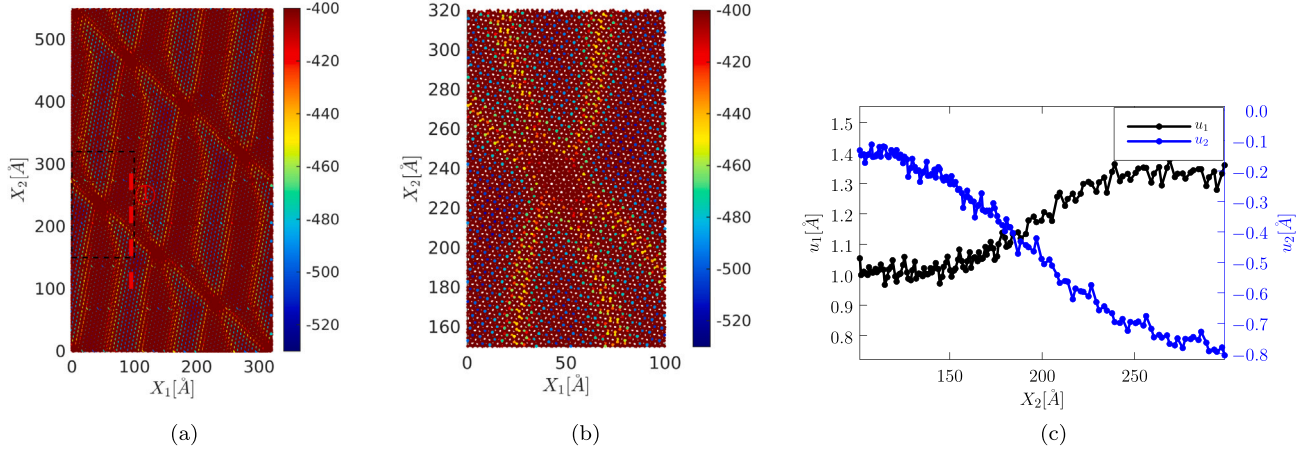
Fig. 6. Atomic reconstruction under a large heterodeformation. (a) Color density plot of atomic energy density [ \text{meV}\text{\AA}^{-2} ] highlighting the network of interface dislocations in a BG heterodeformed relative to the untwisted \Sigma 7 configuration using KC-2 parametrization. (b) A magnified view of the dislocation network in (a). (c) shows variations of the displacement components along the dashed line 1, shown in (a). The displacements are measured relative to the \Sigma 7 configuration.
