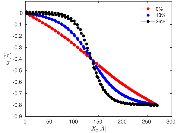
Fig. 5. Burgers Vector for 21.786789^\circ + 0.170076^\circ twisted BG at different magnitudes of out-of-plane compression calculated using the KC-1 parametrization.
