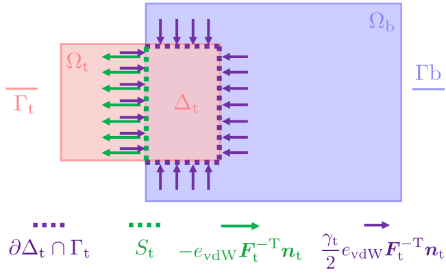
Fig. 13. A schematic showing two types of tractions (purple and green arrows) on the boundary of the overlapping region, \Delta_t \subset \Omega_t , due to surface tension associated with vdW interactions in a finite 2D heterostructure. The traction forces balance the thermodynamic driving forces that act to increase the region of overlap. The purple arrows are compressive forces associated with the overlapping region's tendency to dilate to increase its area. The green arrows are configurational forces on S_t that balance the thermodynamic forces conjugate to aerial changes in \Delta_t due to the translation of \Omega_t into \Omega_b . (For interpretation of the references to color in this figure legend, the reader is referred to the web version of this article.)
