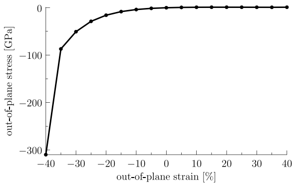
Fig. E.17. The out-of-plane stress vs strain in an AB-stacked bilayer graphene, computed using the KC-1 potential.
