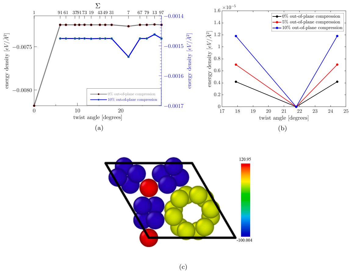
Fig. 3. (a) A comparison of interfacial energy density versus the twist angle of an unrelaxed BG under a 0% and a 10% out-of-plane compression, computed using the KC-1 potential. (b) A similar comparison in the neighborhood of the \Sigma 7 configuration using the KC-2 potential. The \Sigma 7 interfacial energy for each out-of-plane compression was subtracted. (c) Atomic energy density [meV Å -3 ] within a fundamental unit cell of the \Sigma 7 configuration, computed using the KC-1 potential. (For interpretation of the references to color in this figure legend, the reader is referred to the web version of this article.)
