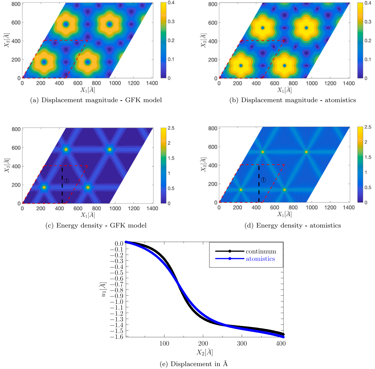
Fig. 14. A comparison of structural relaxation predicted by continuum and atomistics simulations of a 0.29926342507^\circ small-twist BG. The units of energy density and displacement are \text{meV } \text{\AA}^{-2} and \text{\AA} , respectively. The area enclosed by the red dashed line is the simulation domain. (e) compares the displacement across the dashed lines predicted by the atomistic and the FK models. (For interpretation of the references to color in this figure legend, the reader is referred to the web version of this article.)
